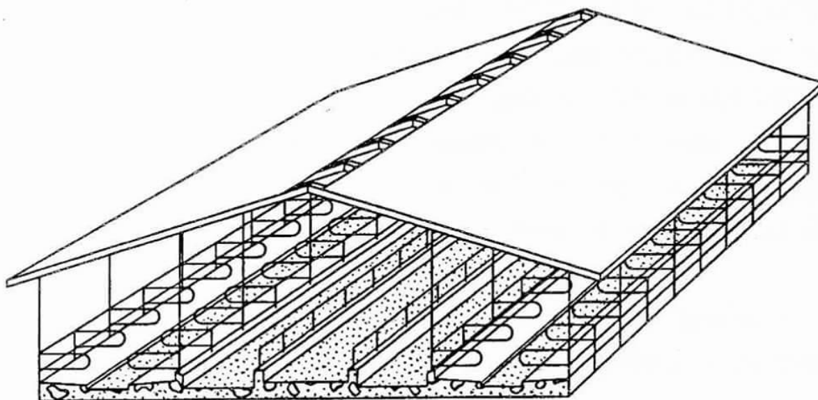
Hot weather with ridge, sidewalls, and endwalls completely opened
