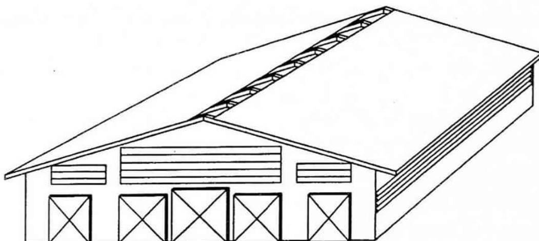
Very cold winter weather with end doors closed and sidewalls opened at least one-half of the ridge width
